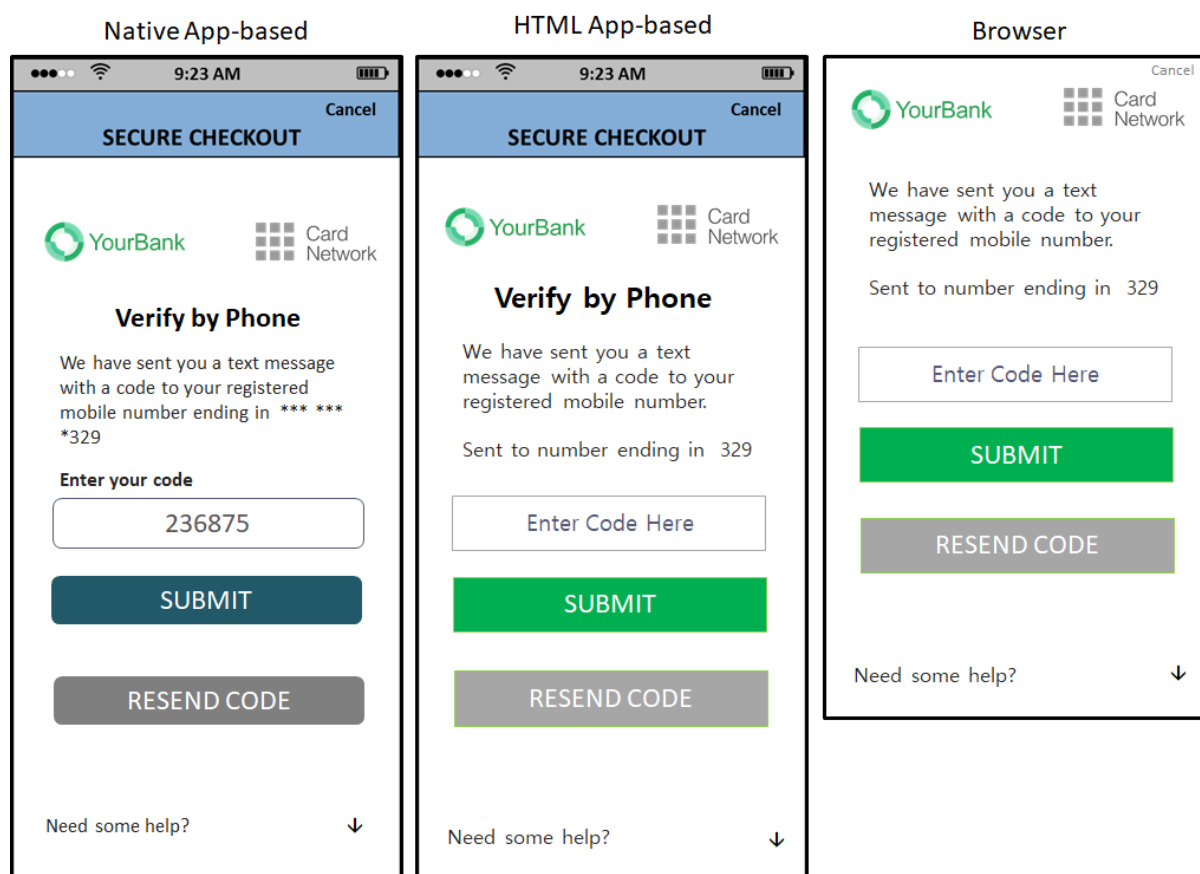
Figure 4.2: UI Template Examples—All Device Channels
