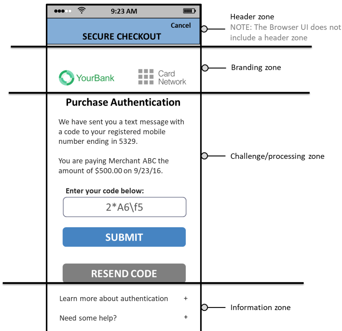
Figure 4.1: UI Template Zones
