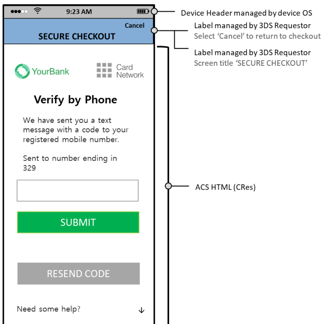
Figure 4.15: Sample HTML UI OTP/Text Template—PA
