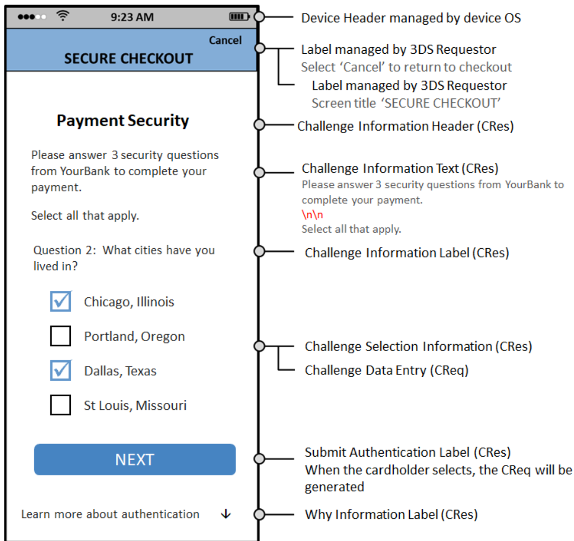
Figure 4.11: Sample Native UI—Multi-select Information—PA
