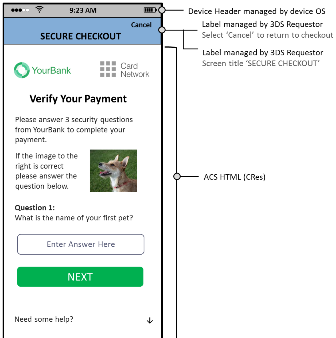
Figure 4.18: Sample HTML Other UI Template—PA
