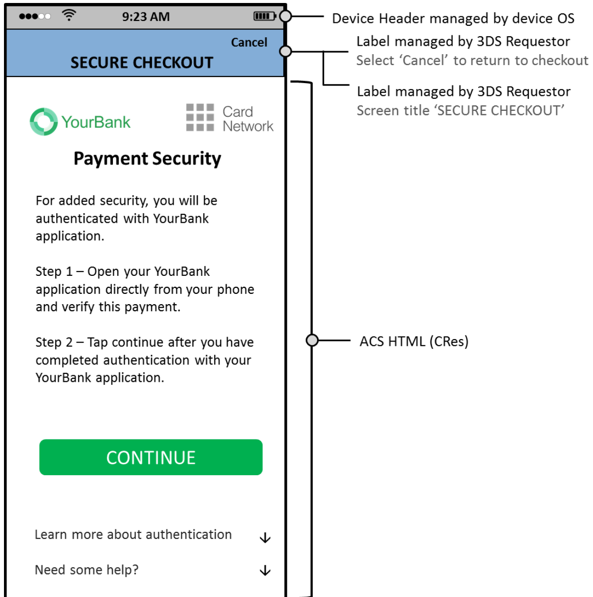
Figure 4.17: Sample OOB HTML UI Template—PA
