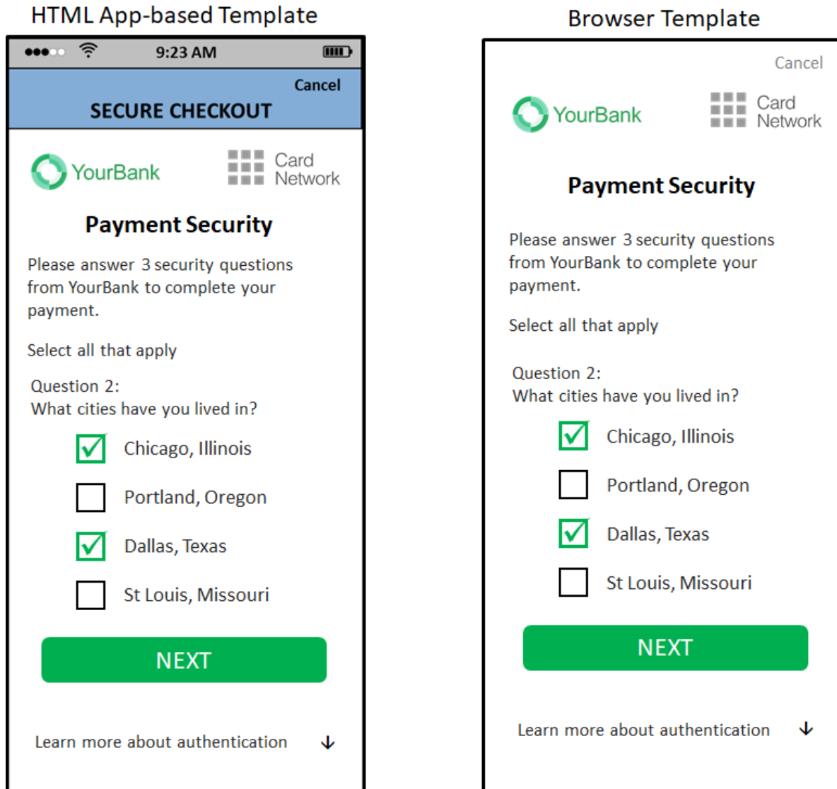
Figure 4.19: App-based HTML and Browser UI Comparison
