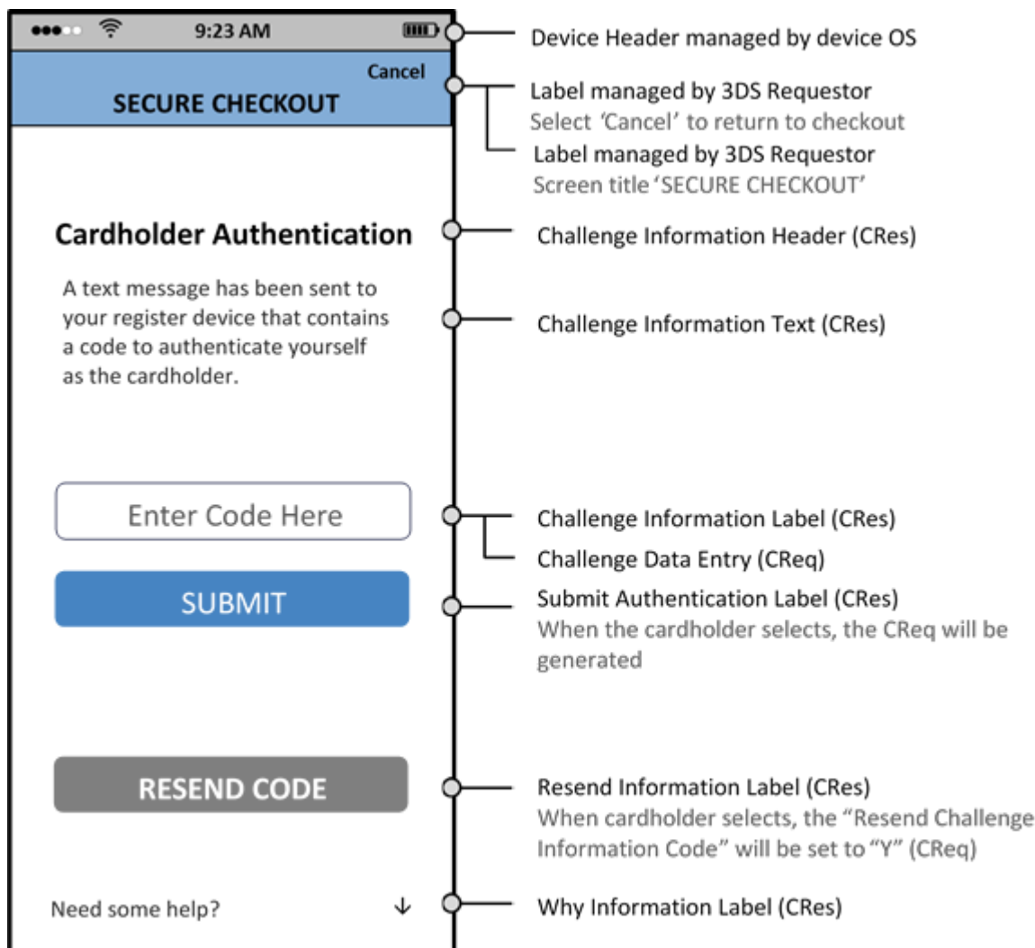
Figure 4.9: Sample Native UI OTP/Text Template—NPA
