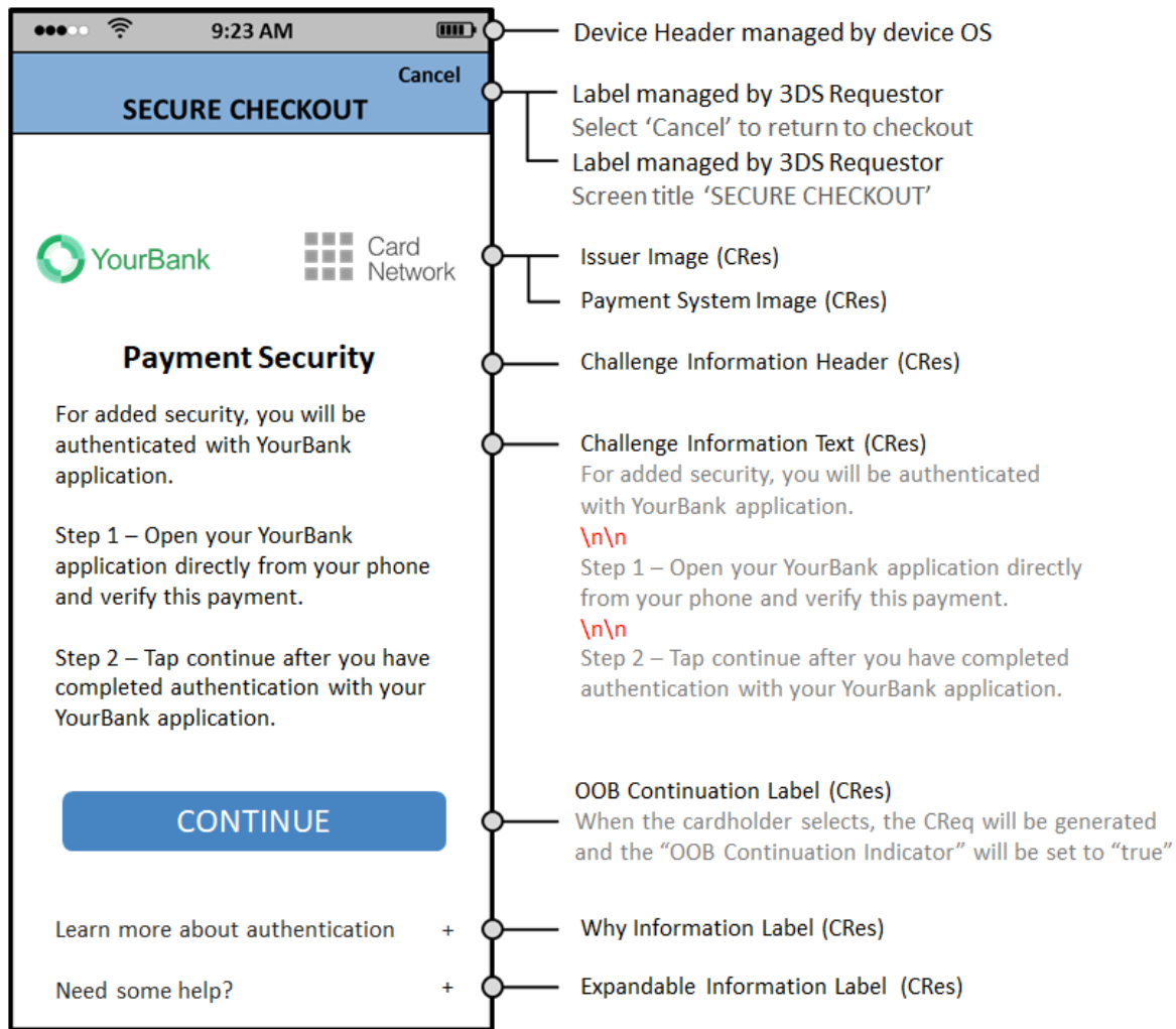
Figure 4.12: Sample OOB Native UI Template—PA
