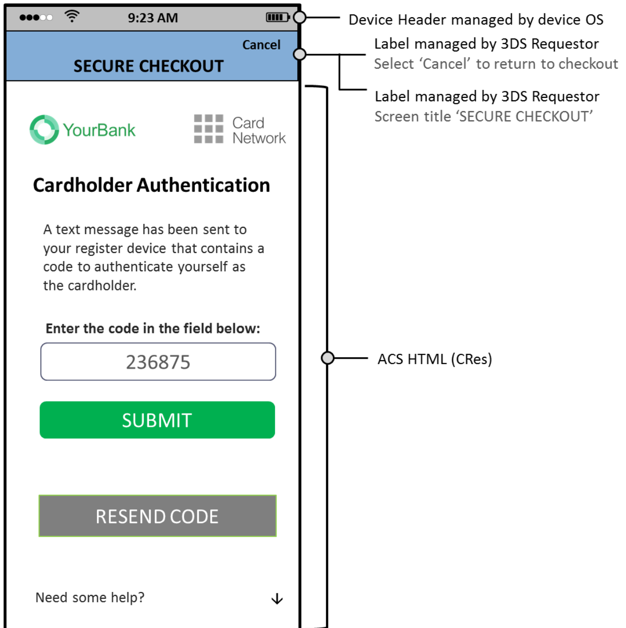
Figure 4.16: Sample UI OTP/Text Template—NPA
