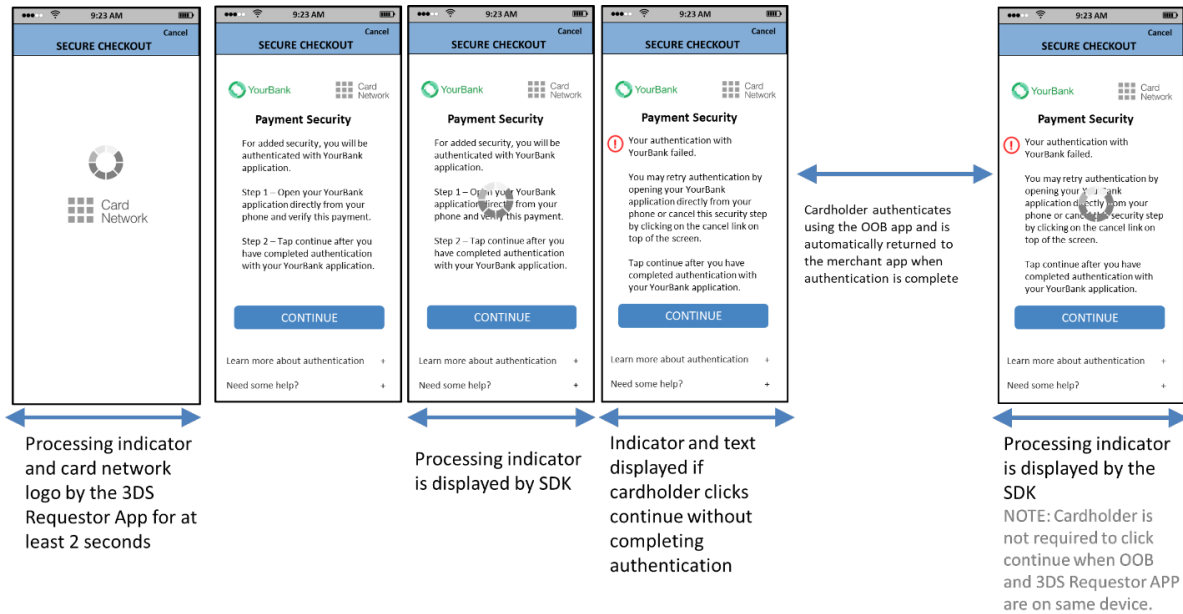
Figure 4.6: Sample OOB Template (OOB App and 3DS Requestor App on same device)—App-based Processing Flow
