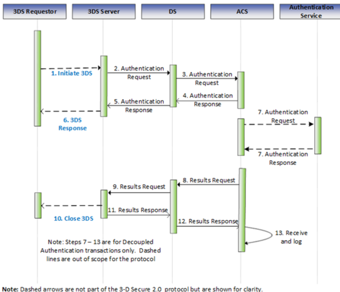
Figure 3.4: 3-D Secure Processing Flow Steps—3RI-based
