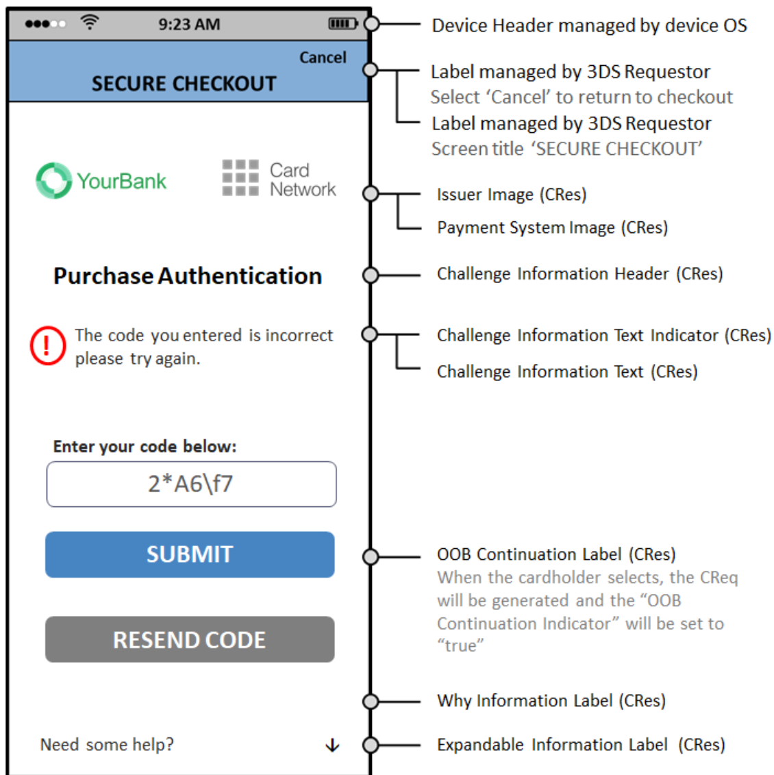
Figure 4.13: Sample Challenge Information Text Indicator—PA
