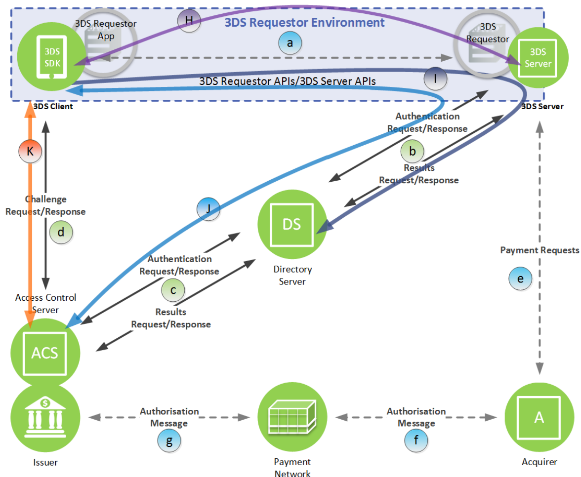
Figure 6.3: Security Functions
