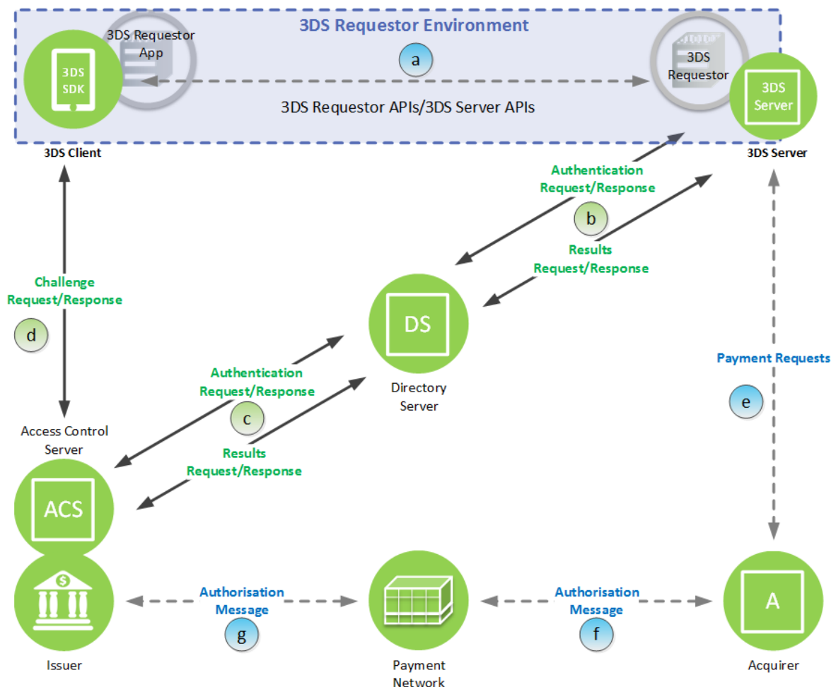
Figure 6.1: Security Flow—App-based
